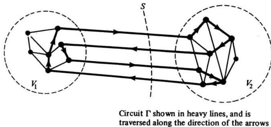
Fig. 4-2 Circuit and a cut-set in G .
