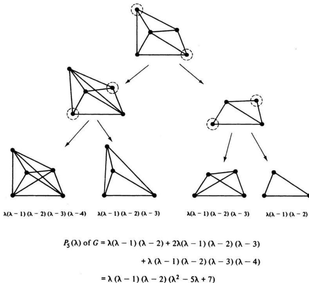
Fig. 8-5 Evaluation of a chromatic polynomial.
